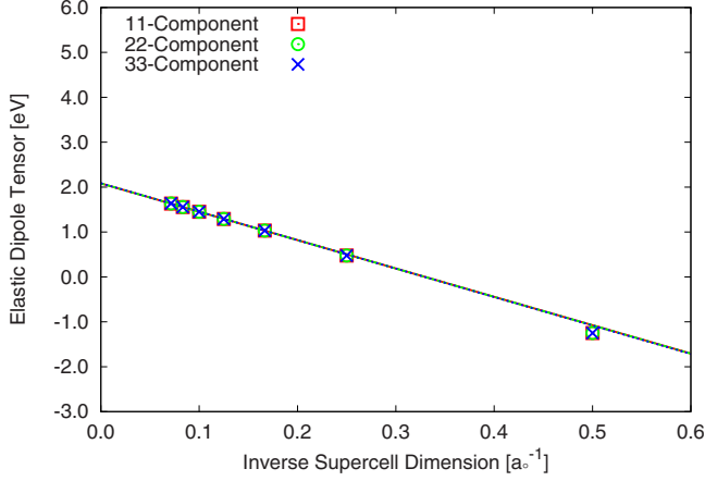
FIG. 4. (Color online) Diagonal components of elastic dipole tensor for strontium vacancy in strontium titanate. Data show linear convergence with inverse linear dimension of supercell size.
