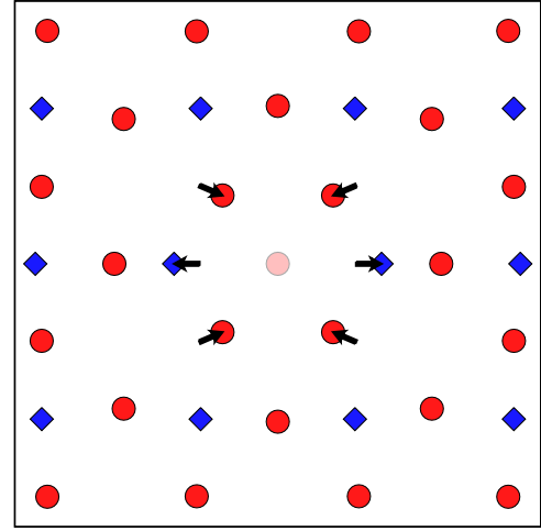
FIG. 3. (Color online) Local strain pattern for oxygen vacancy in the \hat{e}_1\hat{e}_2 plane of strontium titanate: titanium atoms (blue or dark gray diamonds), oxygen atoms (red or gray circles), oxygen vacancy (light red or light gray circle). Atomic displacements exaggerated by a factor of three for clarity (arrows), displayed for significant in-plane displacements ( >0.1 \text{ \AA} ) only.
