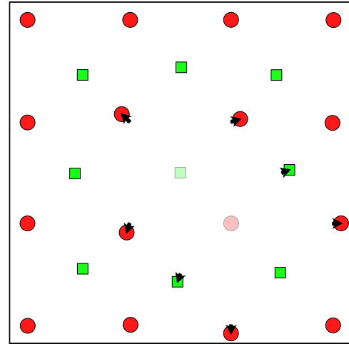
FIG. 9. (Color online) Local strain pattern for strontium-oxygen divacancy in the \hat{e}_1\hat{e}_2 plane of strontium titanate: strontium atoms (green or gray squares), oxygen atoms (red or gray circles), strontium vacancy (light green or light gray square), oxygen vacancy (light red or light gray circle). Atomic displacements exaggerated by a factor of three for clarity (arrows), displayed for significant in-plane displacements ( >0.1 Å) only.
