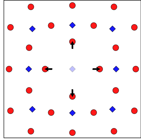
FIG. 7. (Color online) Local strain pattern for titanium vacancy in the \hat{e}_1\hat{e}_2 plane of strontium titanate: titanium atoms (blue or dark gray diamonds), oxygen atoms (red or gray circles), titanium vacancy (light blue or light gray diamond). Atomic displacements exaggerated by a factor of three for clarity (arrows), displayed for significant in-plane displacements ( >0.1 \text{ \AA} ) only.
