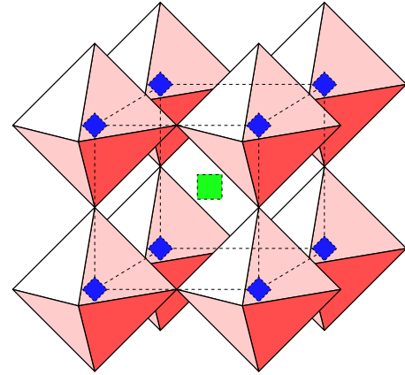
FIG. 1. (Color online) Atomic structure of nonreconstructed cubic strontium titanate: oxygen octahedra surrounding titanium atoms (blue or dark gray diamonds), with strontium atoms (green or gray square) outside the octahedra and equidistant from the titanium sites.
