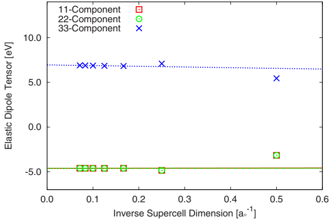
FIG. 8. (Color online) Diagonal components of elastic dipole tensor for strontium-oxygen divacancy in strontium titanate. Data show linear convergence with inverse linear dimension of supercell size.
