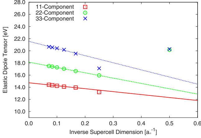
FIG. 10. (Color online) Diagonal components of elastic dipole tensor for titanium-oxygen divacancy in strontium titanate. Data show linear convergence with inverse linear dimension of supercell size.
