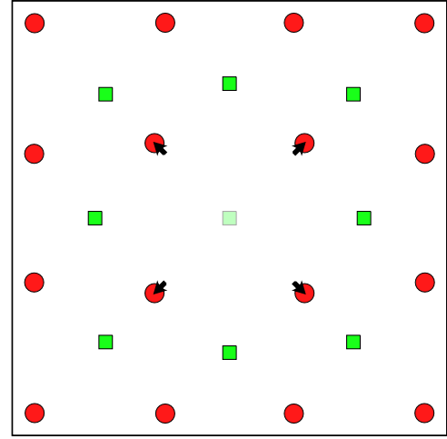
FIG. 5. (Color online) Local strain pattern for strontium vacancy in the \hat{e}_1\hat{e}_2 plane of strontium titanate: strontium atoms (green or gray squares), oxygen atoms (red or gray circles), strontium vacancy (light green or light gray square). Atomic displacements exaggerated by a factor of three for clarity (arrows), displayed for significant in-plane displacements ( >0.1 Å) only.
