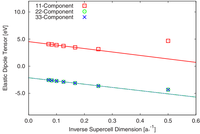
FIG. 2. (Color online) Diagonal components of elastic dipole tensor for oxygen vacancy in strontium titanate. Data show linear convergence with inverse linear dimension of supercell size.
