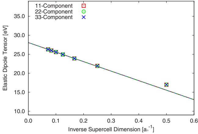
FIG. 6. (Color online) Diagonal components of elastic dipole tensor for titanium vacancy in strontium titanate. Data show linear convergence with inverse linear dimension of supercell size.
