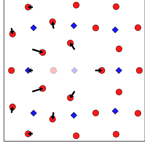
FIG. 11. (Color online) Local strain pattern for titanium-oxygen divacancy in the \hat{e}_1\hat{e}_2 plane of strontium titanate: titanium atoms (blue or dark gray diamonds), oxygen atoms (red or gray circles), titanium vacancy (light blue or light gray diamond), oxygen vacancy (light red or light gray circle). Atomic displacements exaggerated by a factor of three for clarity (arrows), displayed for significant in-plane displacements ( >0.1 Å) only.
